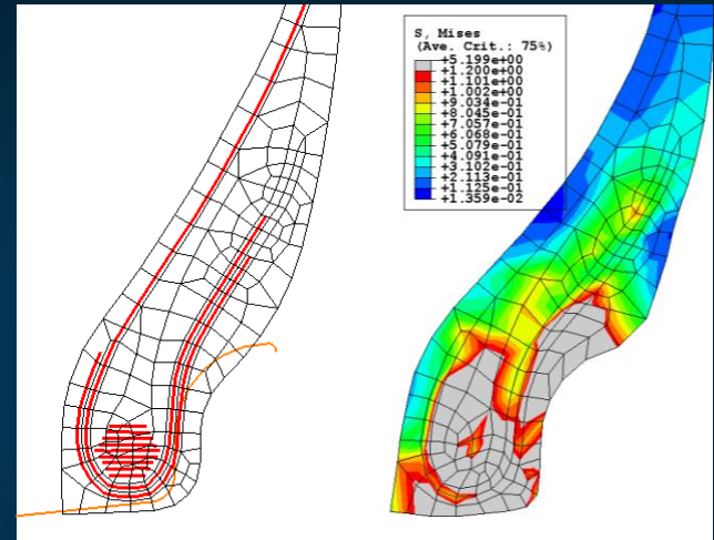
Stress Analysis and Modeling of the Bead
