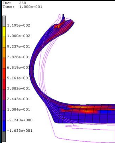
Sidewall Force Deformation Analysis
